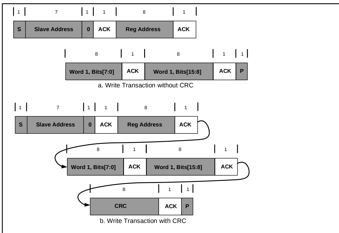
Figure 18: I²C Write Transaction
